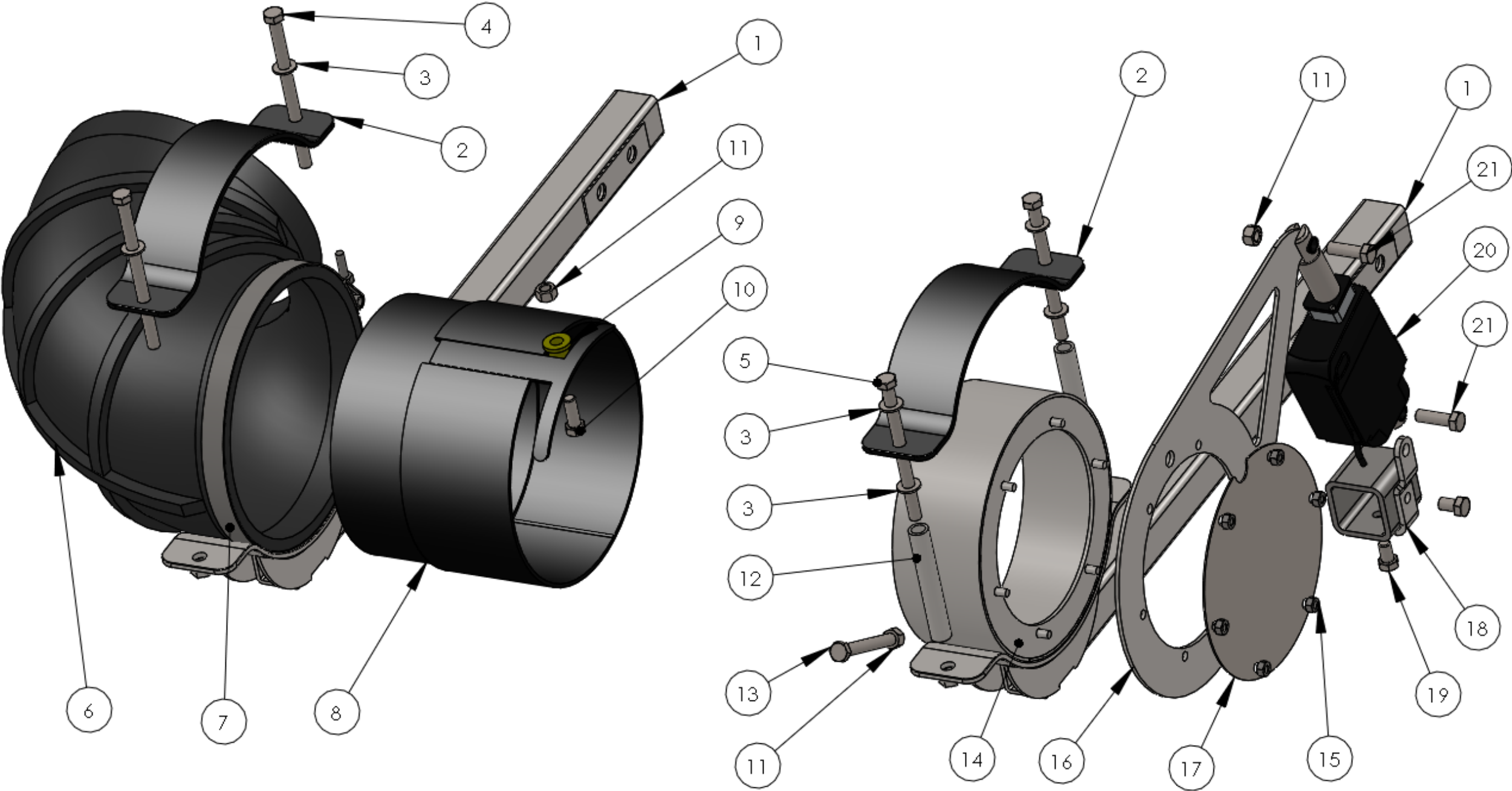
AWS0814 End Cap Assembly, w/ lever includes items 11,13,14,15,16,17 and replaces AWS0094 End Cap (-2015)
