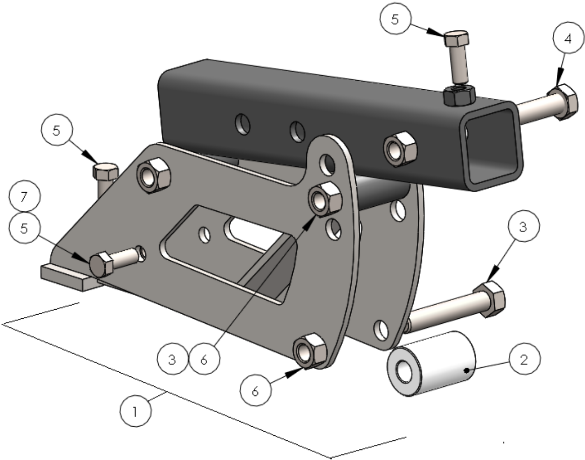
Centre Bracket
