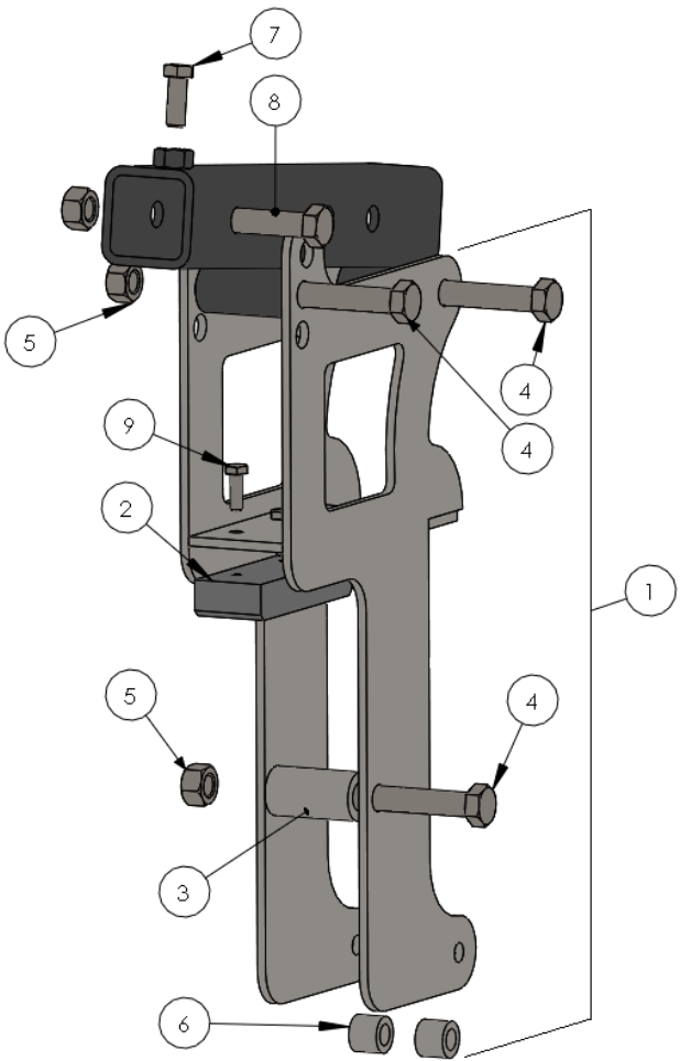
JD 635FD Mount Arm, Left
