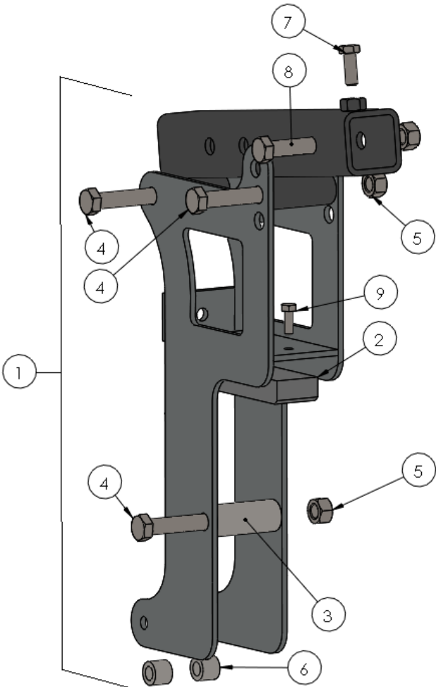
JD 635FD Mount Arm, Right
