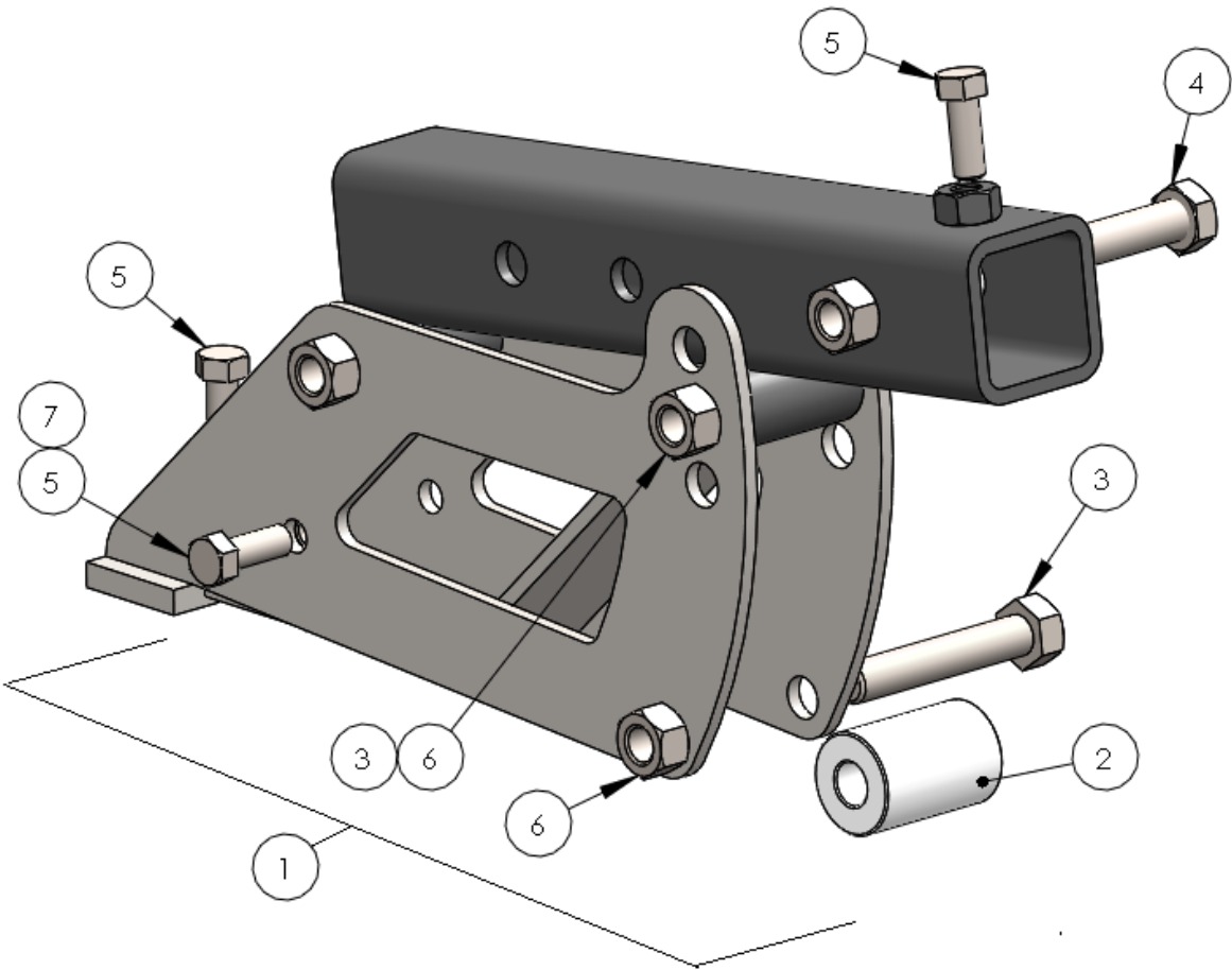
Centre Bracket
