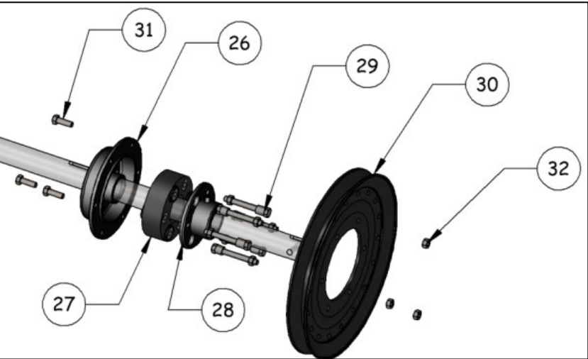
AWS0350 Knife Drive Assy. Optional (50 series combines)
